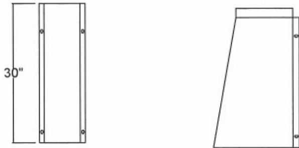
97 Series PILASTER Elevation
